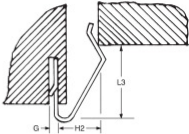
TYPICAL ASSEMBLY
